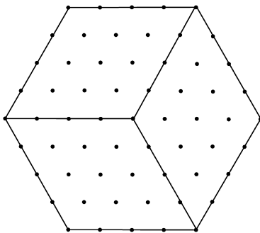
Figure 2.1 Dots on a cube
